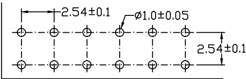
Recommend PCB Layout
